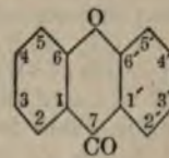
Xanthone.
